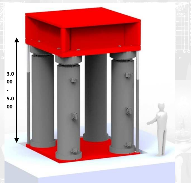
Monoaxial press of 30 MN: 2.000 mm stroke
